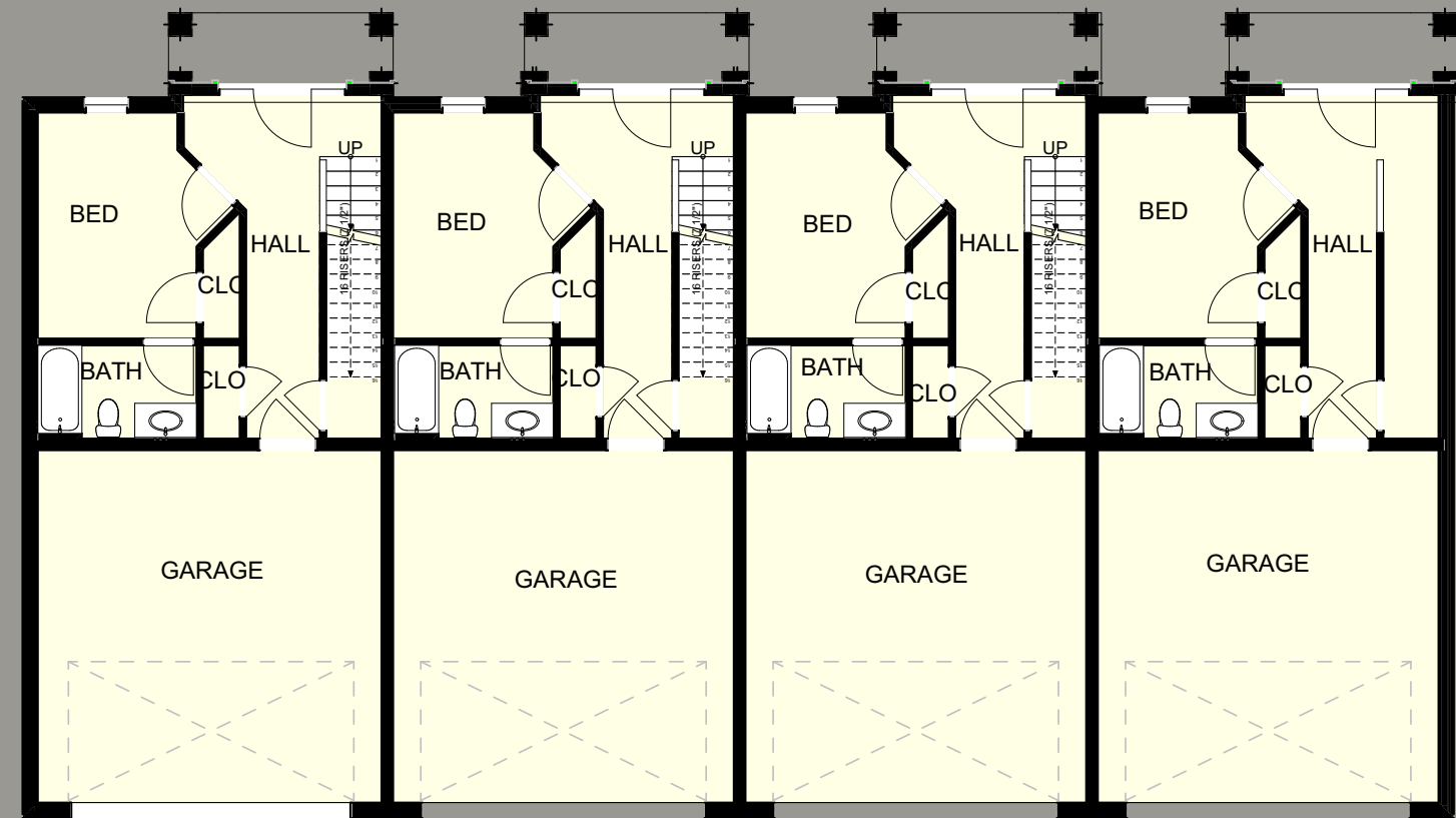
3-story Options - GROUND FLOOR PLAN
