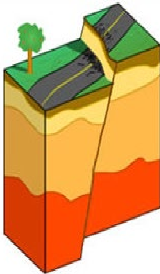
Normal fault
