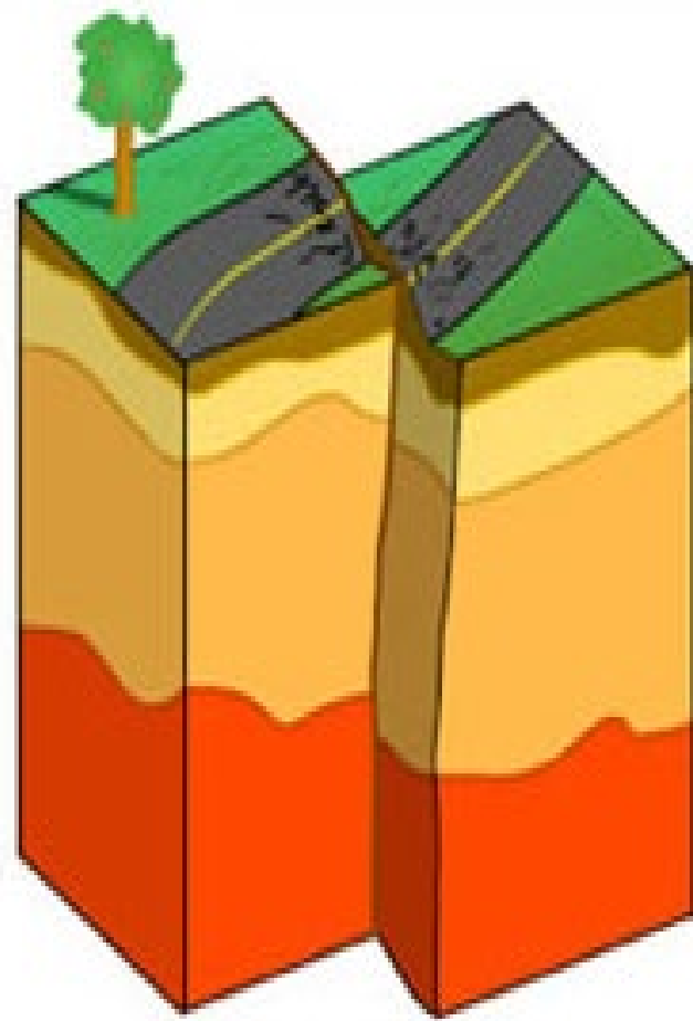
Strike-slip fault
