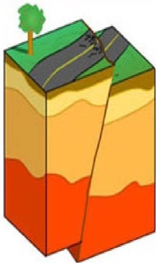
Reverse fault
