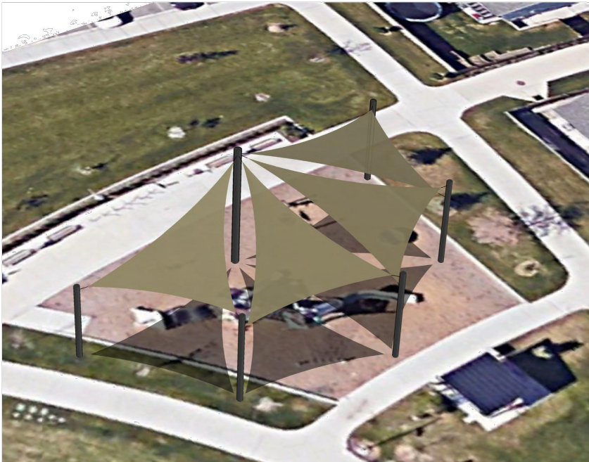
PERSPECTIVE VIEW
