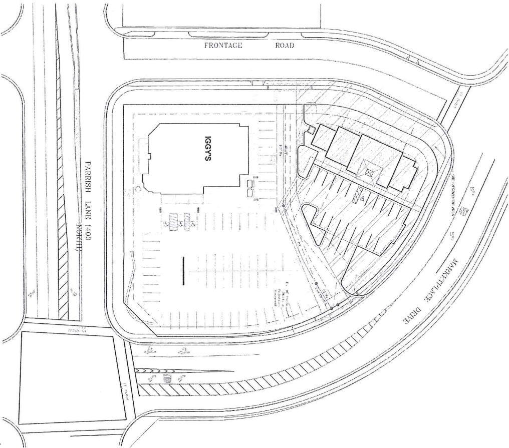
SITE PLAN 1" = 30' 0"
